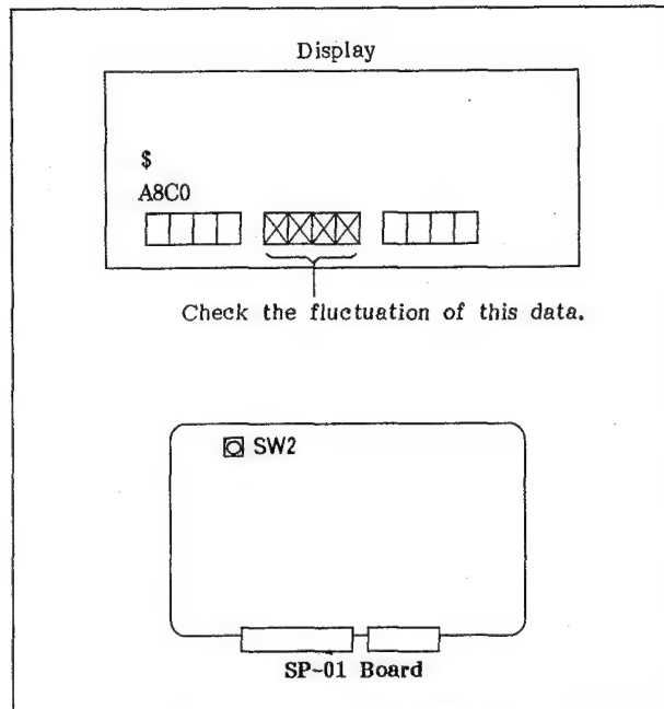
Fig. 9-10 Tape Speed Adjustment
